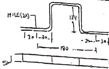
BACK CLAMP 50 X 6 X 484 MM
