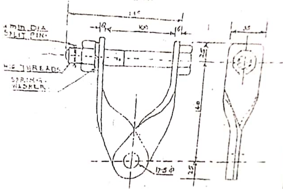
CROSS-ARM STRAPS
