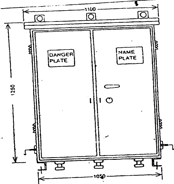
FRONT - VIEW WITH DOOR
