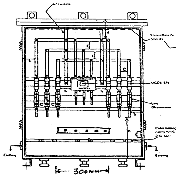
BACK & FRONT VIEW WITHOUT DOOR
