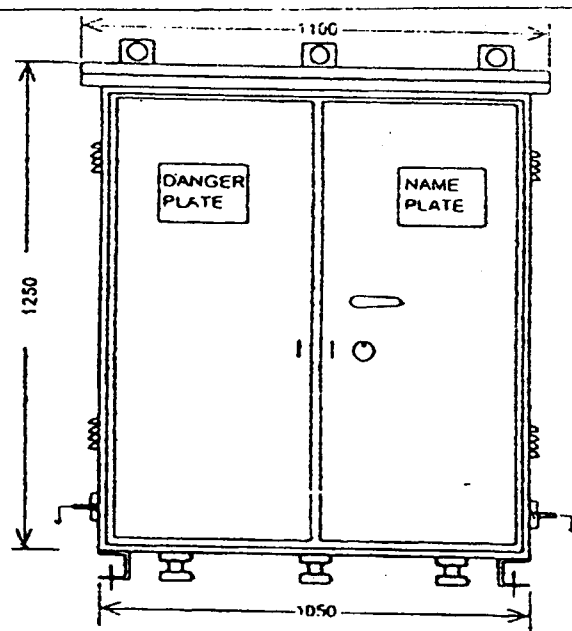
BACK & FRONT VIEW WITH DOOR
