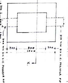
P.L. PLAN (OIL MAN HOLE)
